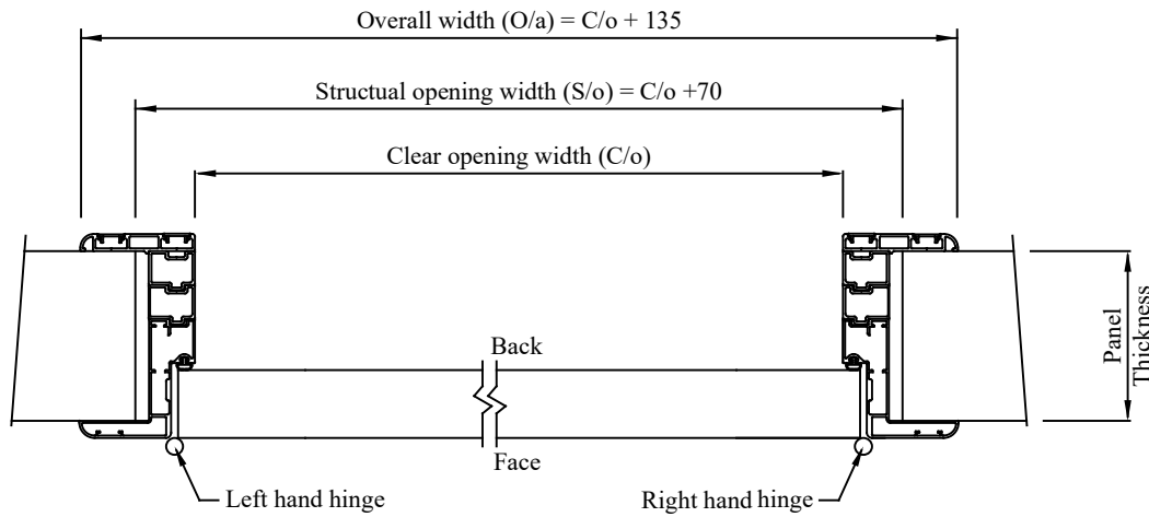
Horizontal section
